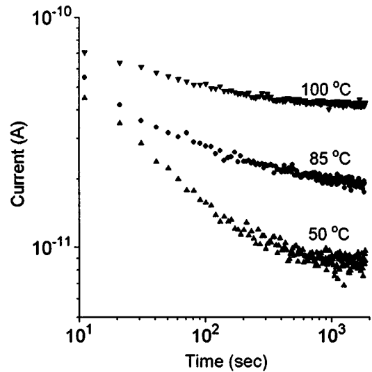
FIG. 3. Conduction currents at 25 MV/m as a function of time at various temperatures.
