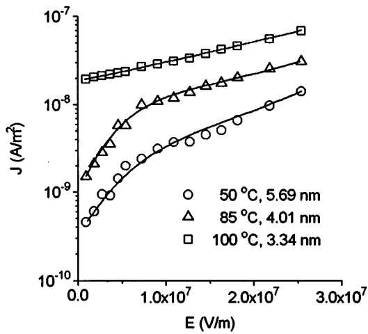
FIG. 5. Comparison of measured and calculated current densities as a function of electric fields: Measured data (symbols), calculated data (solid line).
