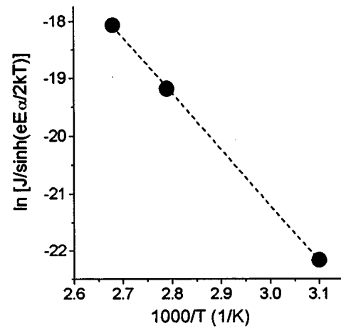
FIG. 6. Temperature dependence of current densities in PEI.
