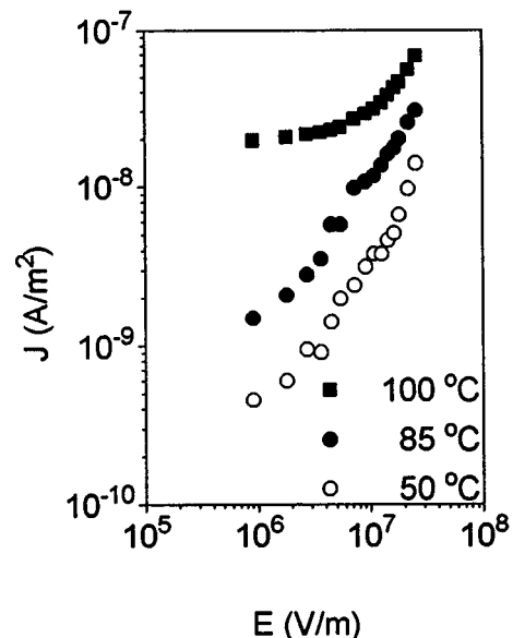
FIG. 4. J - E curves of PEI after 1800 s.
