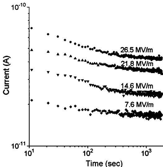
FIG. 2. Conduction currents at 100 °C as a function of time at various electric fields.
